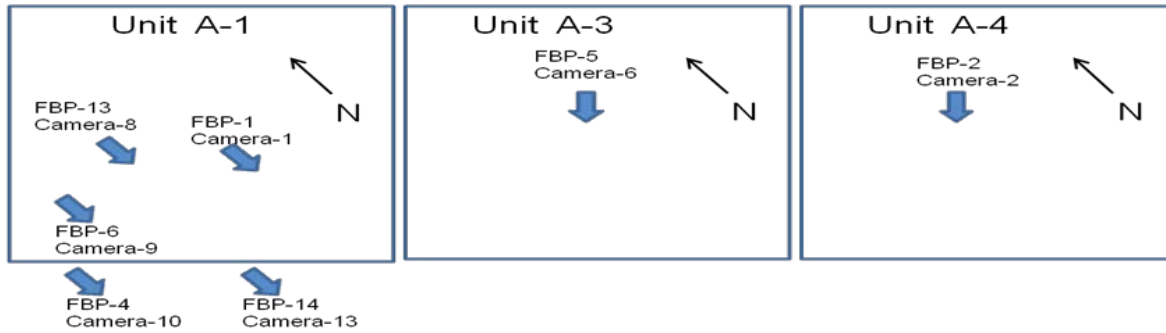
Figure 4 – Layout of sensors in burn unit.
