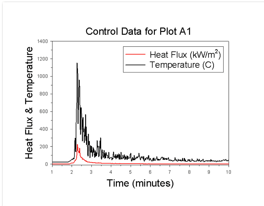
Figure 13. Temperature and heat flux data from unit A-1.
