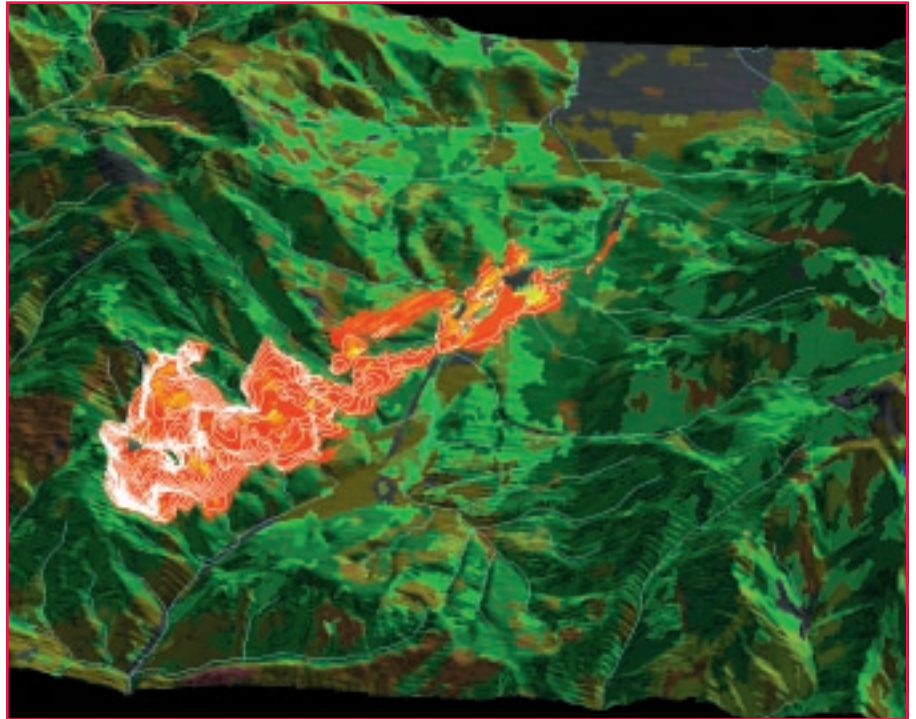
Figure 1—A FARSITE display using ArcView 3.0 to show fire intensity and perimeter output. FARSITE's spatial maps of fire behavior can help produce detailed analyses of fire behavior and fire effects.
