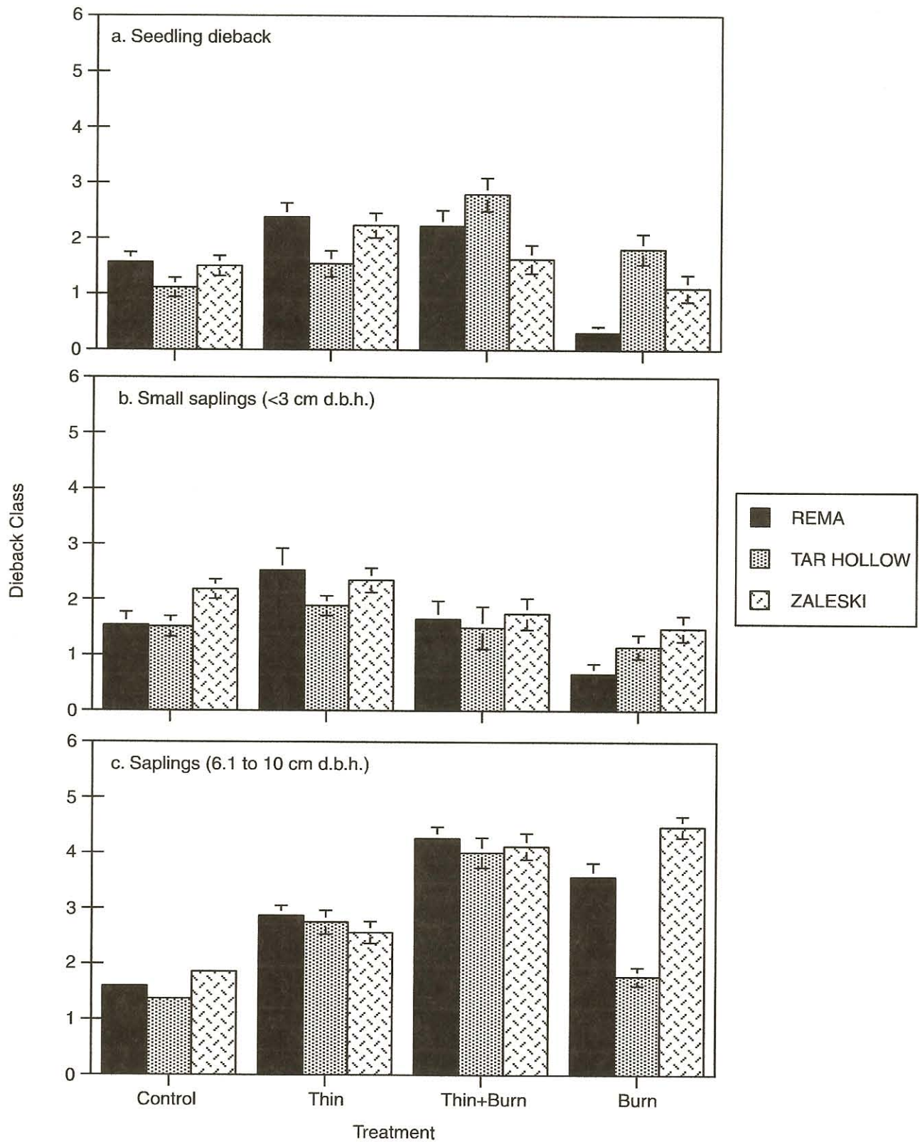
Figure 5—Late summer assessments of dieback of hardwood seedlings and saplings following prescribed fires and/or overstory thinning: (a) mean seedling dieback per plot; (b) mean small sapling dieback per plot; and (c) mean sapling dieback per plot. Rating of 1 = <10 percent dieback, while a rating of 5 = 76 to 100 percent dieback.
