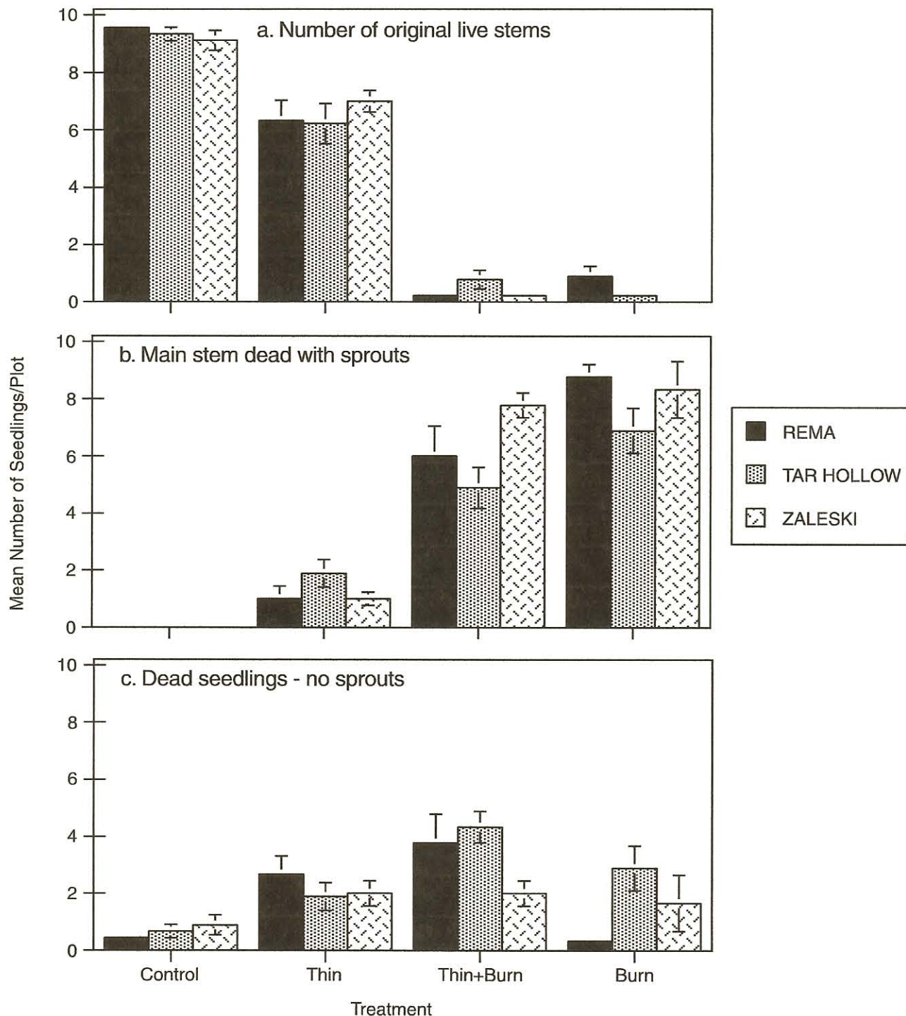
Figure 2—Survival of oak and hickory seedlings 4 months after low-intensity prescribed fires and/or overstory thinning at three sites in southern Ohio: (a) mean number of original live stems per plot; (b) mean number of dead stems with live sprouts per plot; (c) mean number of dead seedlings with no live sprouts.
