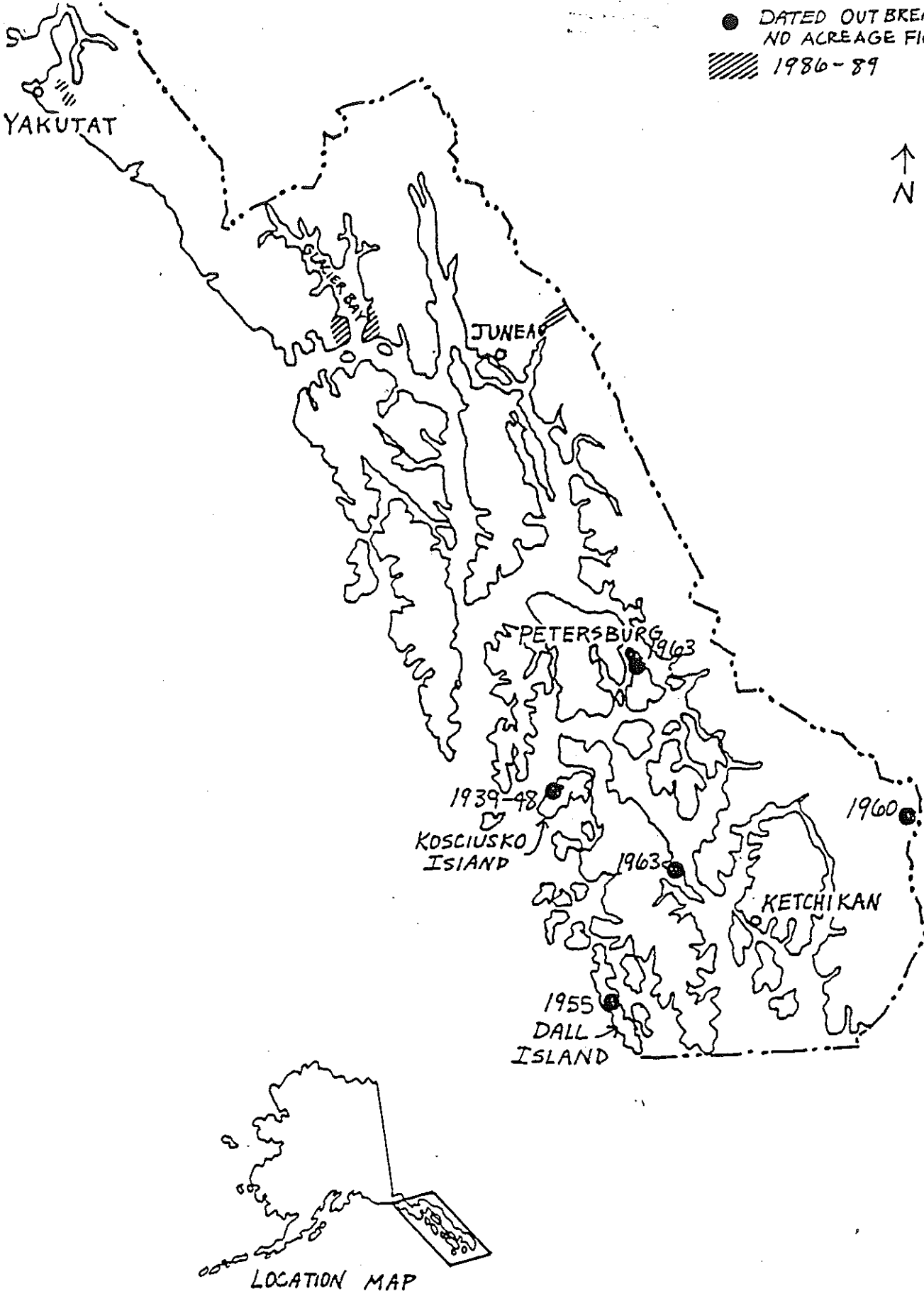
Figure 2b. Location of spruce beetle outbreaks in southeast Alaska's maritime Sitka spruce stands.
