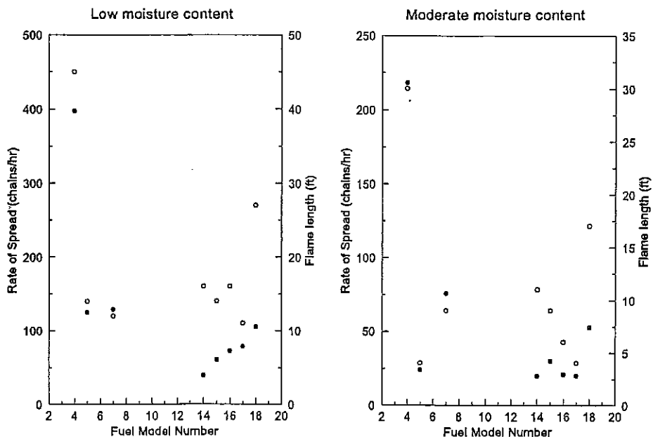
Figure 1. Rate of spread (ROS) and flame length (FL) predictions from TSTMDL for custom chaparral and FBPS fuel models for low and moderate fuel moisture conditions. solid circles are ROS predictions, empty circles are FL predictions.
