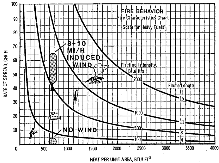
Figure 11. Indraft effect upon sage brush fire characteristics.
