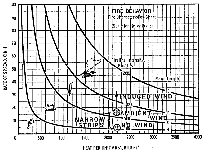
Figure 12. Indraft effect upon logging slash fire characteristics.
