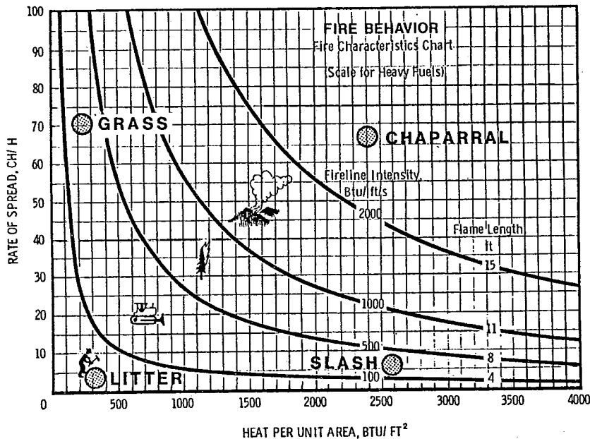
Figure 10. Fire characteristics chart.
