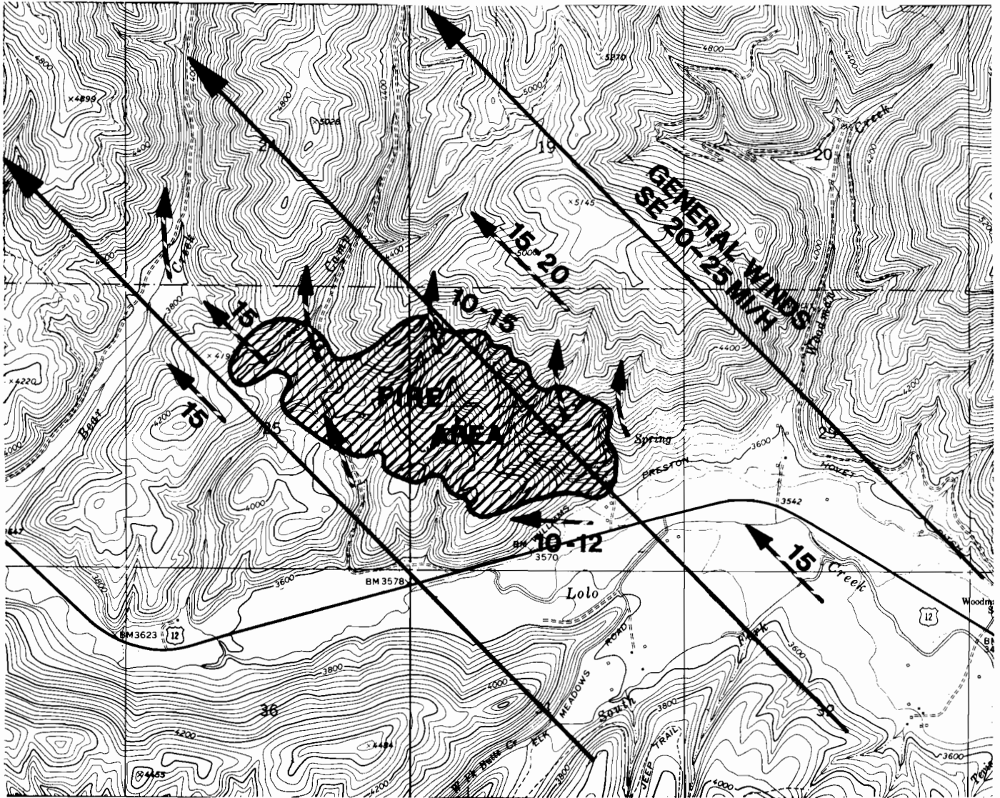
Figure II-7.—Diagrammatic layout of local winds as influenced by topography.
