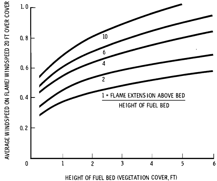
Figure B-1.—Average windspeed acting on a flame extending above a uniform surface fuelbed layer (vegetation cover), due to log windspeed variation.
