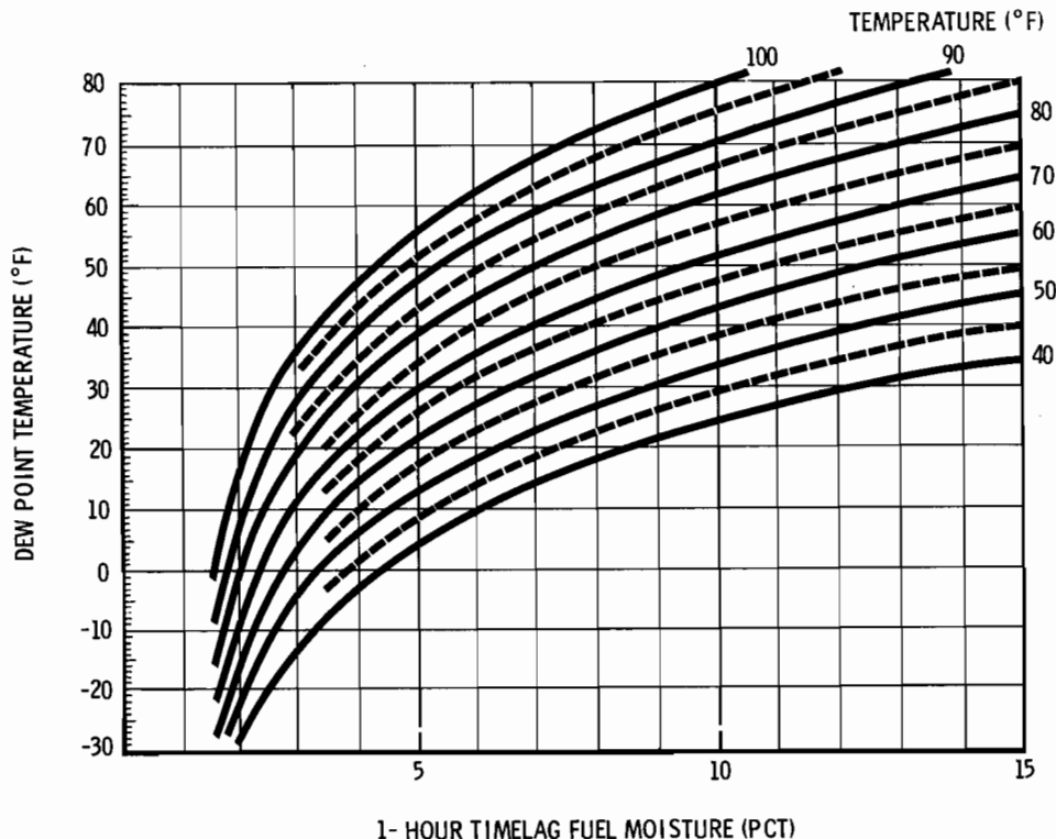
Figure D-1.—Elevation correction of 1-hour timelag fuel moisture.
