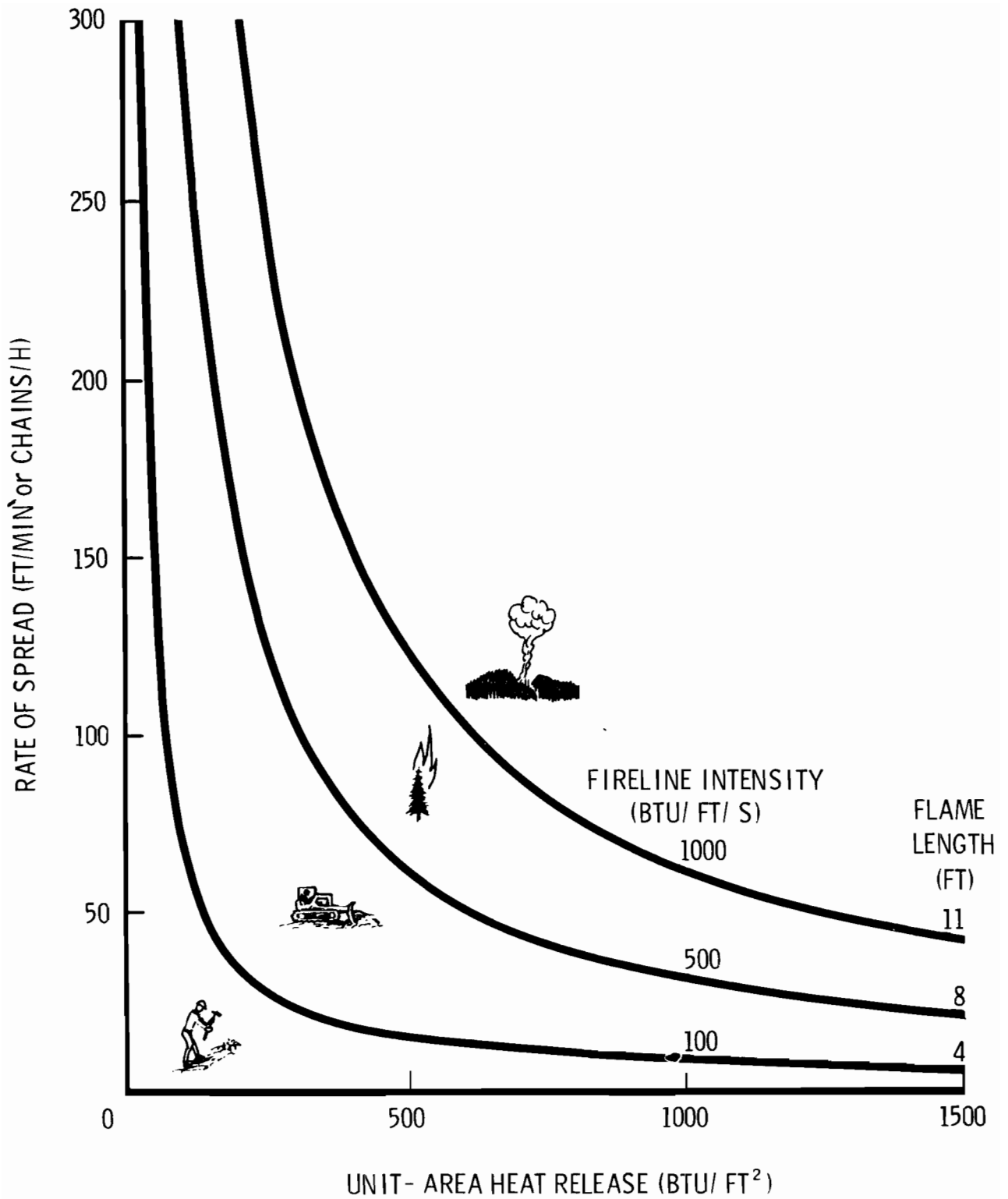
Figure 2.--The potential spread rate and intensity of a fire can be characterized by plotting unit-area heat release and rate of spread.
