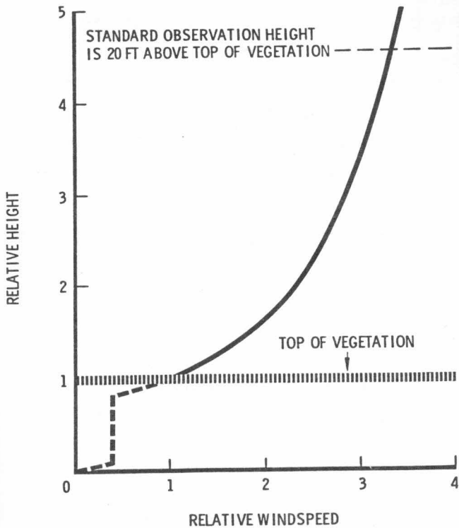
Figure 1.--Wind profile.
