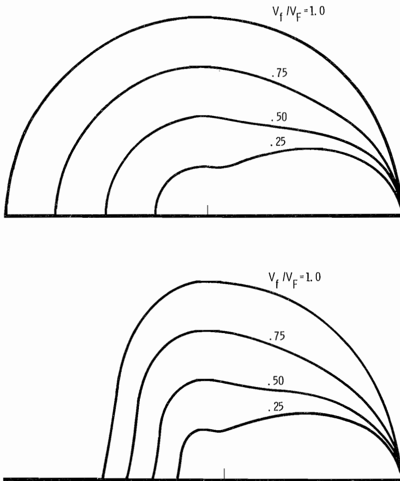
Figure 2.--Shapes of fires generated by equation 9. In all cases, the fire perimeter is drawn to a scale such that the distance from the point of ignition (tick mark on horizontal line) to the head of the fire (right-hand edge of each outline) is the same. In the upper figure V_B/V_f = 1.0 ; in the lower figure V_B/V_f = 0.5 ; for both figures n = 4 .
