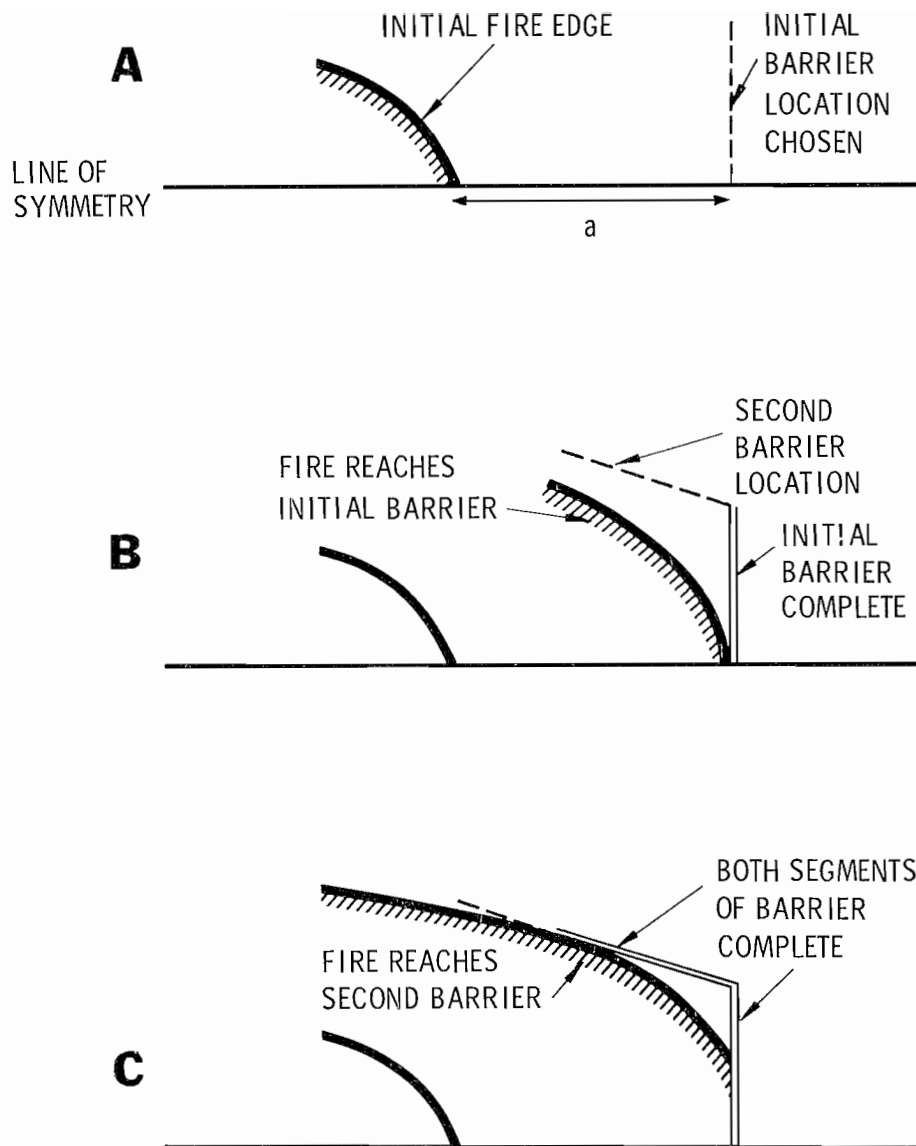
Figure 4A.--The first step in controlling a rapid head fire is the construction of a barrier at distance "a" ahead of the initial fire location. B: Construction of the second segment of the barrier starts when the fire reaches the first segment. C: Work proceeds against the flanking fire, by direct attack, when the fire reaches the second barrier segment.
